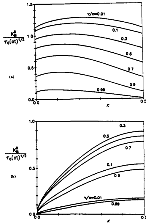
Fig. 5. Symmetric crack bifurcation ( \kappa_1 = -\kappa_2 = \kappa , v_1 = v_2 = v ): (a) \alpha = 0 (normal incidence), K_{III}^P = K_{III}^C vs \kappa ; (b) \alpha = 0.5 (grazing incidence), K_{III}^P = -K_{III}^C vs \kappa .
